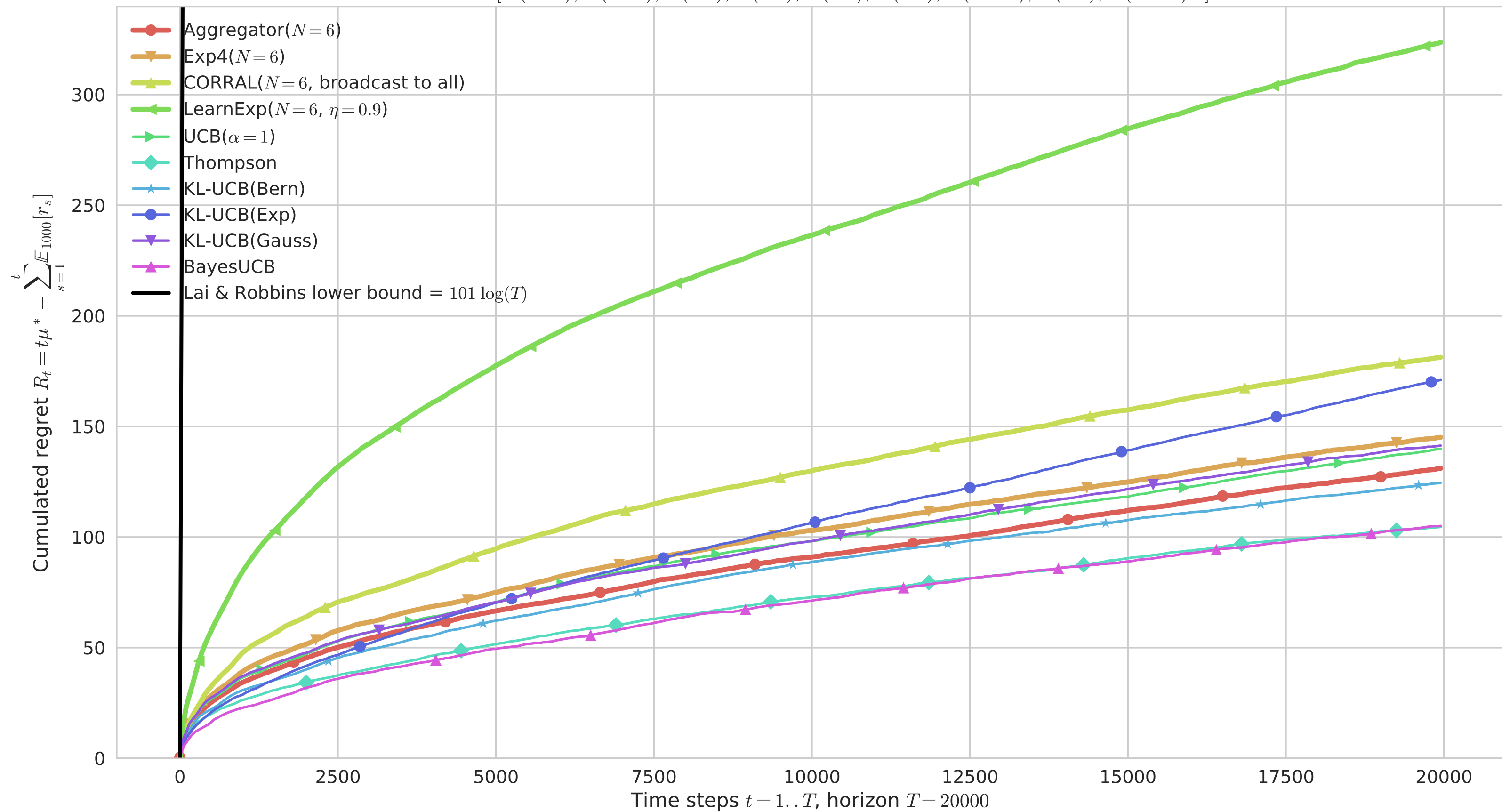
Cumulated regrets for different bandit algorithms, averaged 1000 times 9 arms: [B(0.01), B(0.02), B(0.3), B(0.4), B(0.5), B(0.6), B(0.795), B(0.8), B(0.805)^*]
